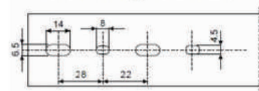
Bottom Mounting Slot Dimensions
